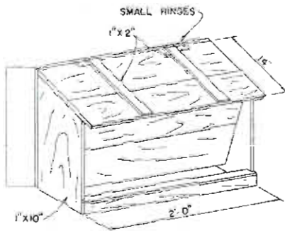
PERSPECTIVE
