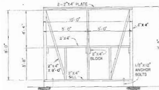
FRONT FRAMING
