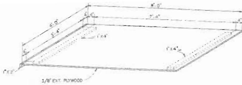
ROOF
