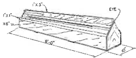
PERSPECTIVE
