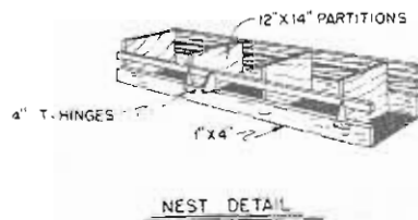
Nest section and detail for 20' x 20' Layer House
