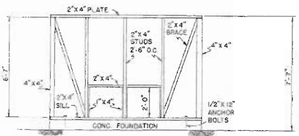
REAR FRAMING
