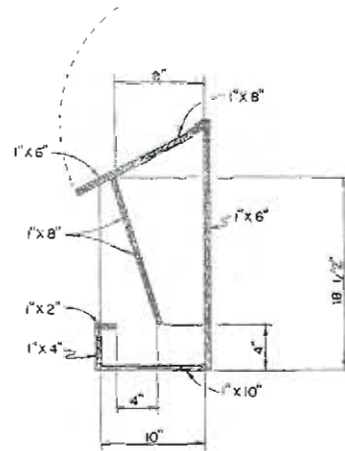
SECTION
