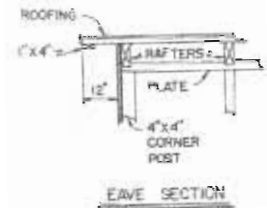
EAVE SECTION
