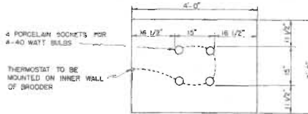
ELECTRICAL LAYOUT FOR BROODER
