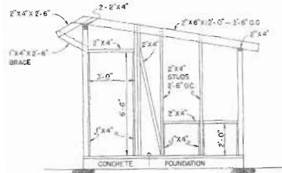
SIDE FRAMING
