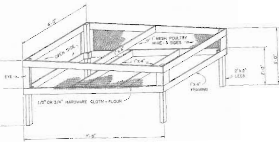
SUN PORCH
